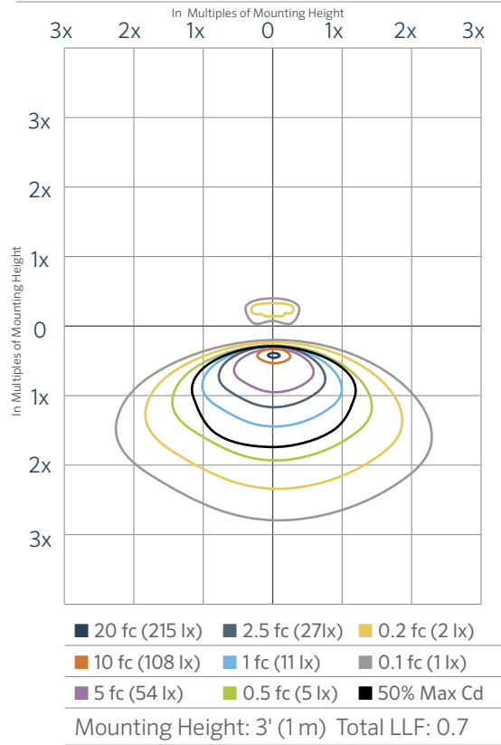
A-BR10 L10 GV Isofootcandle Plot
