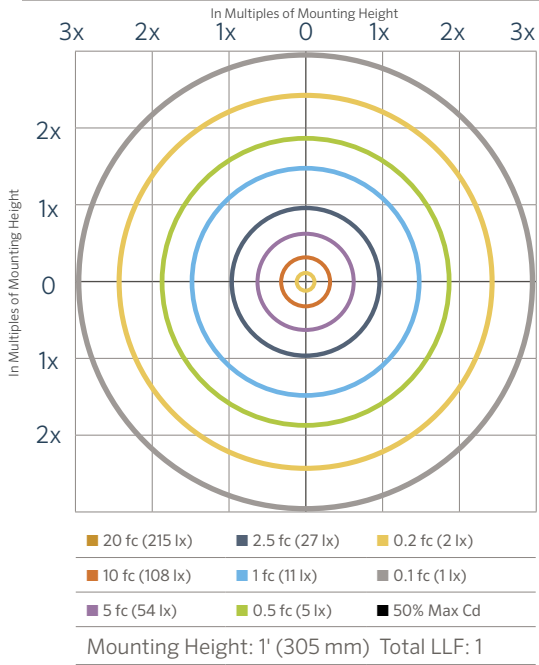
PR 1LED Isofootcandle Plot
