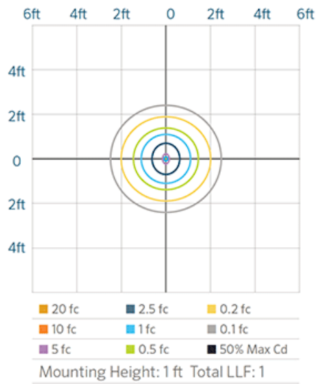
DM LED 10W ISOFOOTCANDLE PLOT
