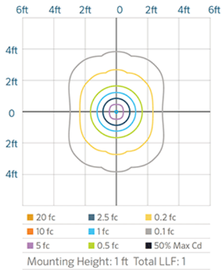
DM LED 20W ISOFOOTCANDLE PLOT
