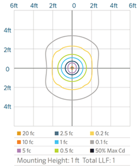
PL LED 20W ISOFOOTCANDLE PLOT
