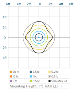
SP LED 10W ISOFOOTCANDLE PLOT
