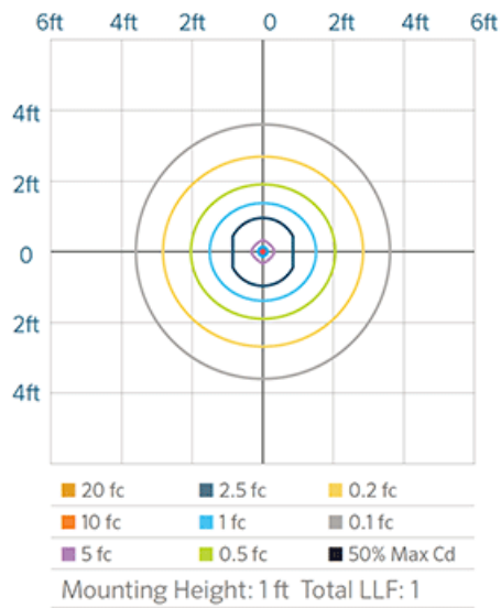
PL LED 10W ISOFOOTCANDLE PLOT
