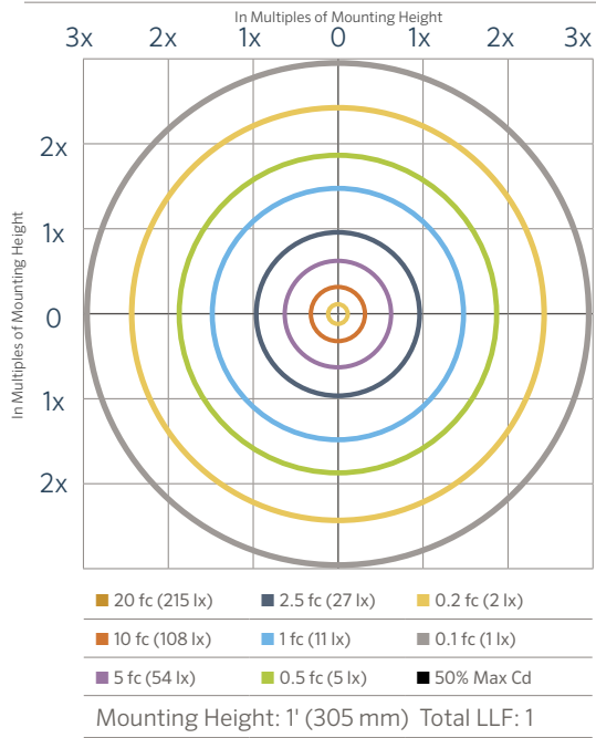
SC 1LED Isofootcandle Plot
